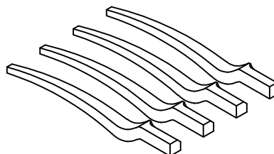
Ref: B - Legs Dimension (mm): 765x76x76 Quantity: 4 pcs Box Number: 1
